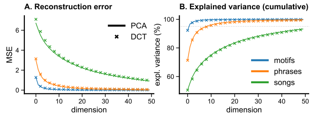
Figure 3. DCT approximates PCA, the optimal transform, in terms of the reconstruction error (A) and the explained variance ratio (B). The reconstruction error is the mean squared error between an contour and a lower dimensional reconstruction. Note that data corresponds to figure 2, and that we did not discard the first component c_0 of the DCT in this figure.
